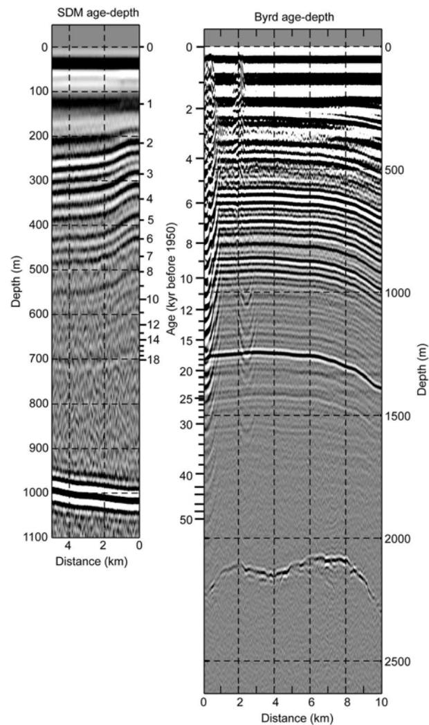
Fig. 4. Detail of radar profiles near the Byrd Station and Siple Dome core sites with superposed age–depth scales nearest the core locations (see text for references). The profiles are scaled vertically to match at 0 and 18 kyr. The deepest observed layer at Siple Dome is very close in age to the bright layer at Byrd Station near 17.5 kyr.
