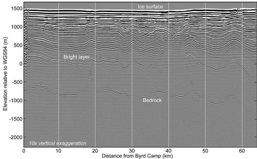
Fig. 2. Radar data processed and migrated as an elevation section from the 2002 US-ITASE traverse. Byrd Station is at the left and the traverse extends in the general direction of South Pole to the right. The bright layer is seen at approximately 1260 m depth near the station. Hyperbolic echoes near Byrd Station are from buried debris associated with relict camp structures. Note the rough bed topography in the vicinity of the camp, and the brightness of the layer which rivals bed echo amplitudes.
