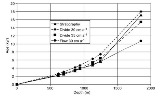
Fig. 5. Age–depth relationship at the inland WAIS divide location (solid line) inferred from layer tracing and the age–depth scale at Byrd Station. Also shown are three model calculations (dashed lines) of the age–depth curve based on assumed average accumulation rates of 30–35 cm a −1 (ice equivalent) and either a constant divide location or steady-state flow on a divide flank.
