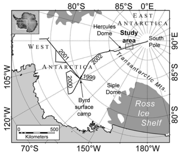
Fig. 1. Map of the 1999–2002 US-ITASE routes in West and East Antarctica, highlighting the study area between Hercules Dome and South Pole.
