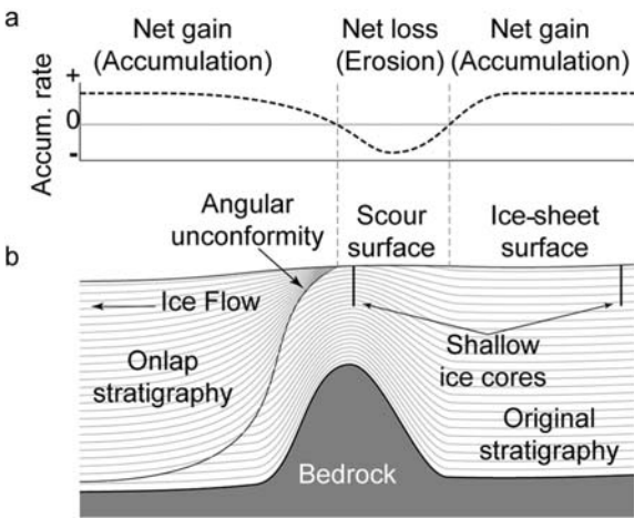
Fig. 6. (a) Hypothetical accumulation rate distribution (heavy dashed line) over an ice surface rise caused by ice flow over a large bedrock mountain. (b) Cartoon of along-flow ice stratigraphy over a bedrock mountain where erosion of surface snow causes an unconformity that is subsequently advected and buried downstream. A shallow ice core at the scour zone could access older ice than the well-dated core located upstream. The age–depth relationship of the pristine upstream core is tied to the scour core using RES profiles.
