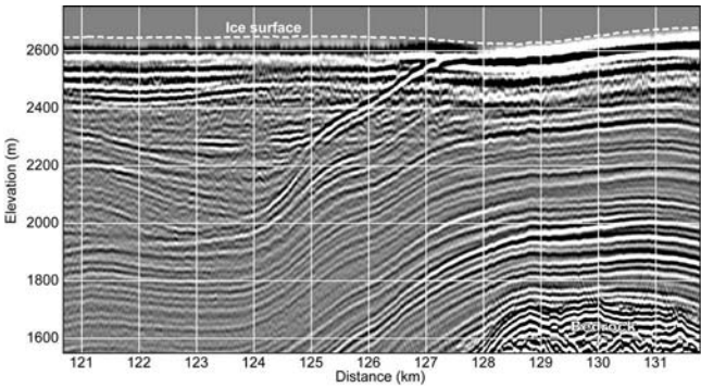
Fig. 4. Close-up of cross-cutting reflector seen in elevation section of 3 MHz radar data. The reflector is nearly conformable to deeper layers but cross-cuts overlying stratigraphy, leading to the interpretation as an angular unconformity. The top of the basal mountain is seen at the lower right. Vertical exaggeration is 5×.
