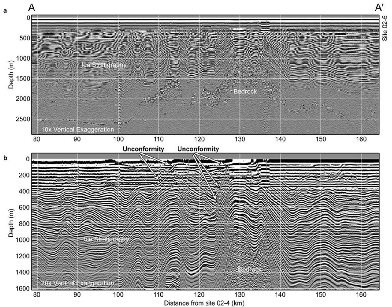
Fig. 3. (a) Processed RES data from profile A–A' plotted with 10× vertical exaggeration. (b) Near-surface stratigraphy shown after horizontal filter to remove much of surface ringing. The strongest two cross-cutting internal reflectors are seen at km 115 and km 128. The horizontal filter adds some noise at greater depths (e.g. at 825 m depth).
