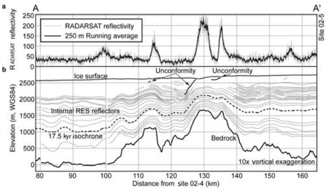
Fig. 5. (a) Interpolated RADARSAT reflectivity values from profile A–A'. The RADARSAT data were smoothed with a 250 m running average. (b) Interpretation of RES data along profile A–A' ending at ice-core site 02-5. Data were geolocated and elevation-corrected using concurrent precision GPS measurements. The bedrock topography (heavy black line) shows a large bedrock mountain approximately 1700 m in elevation. Internal stratigraphy (thin gray lines) is generally conformable to the bedrock topography and ice surface. A prominent angular unconformity intersects the ice surface near km 128.
