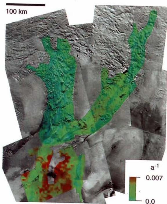
Fig. 8. Error (one- \sigma ) in longitudinal strain rate (color).
