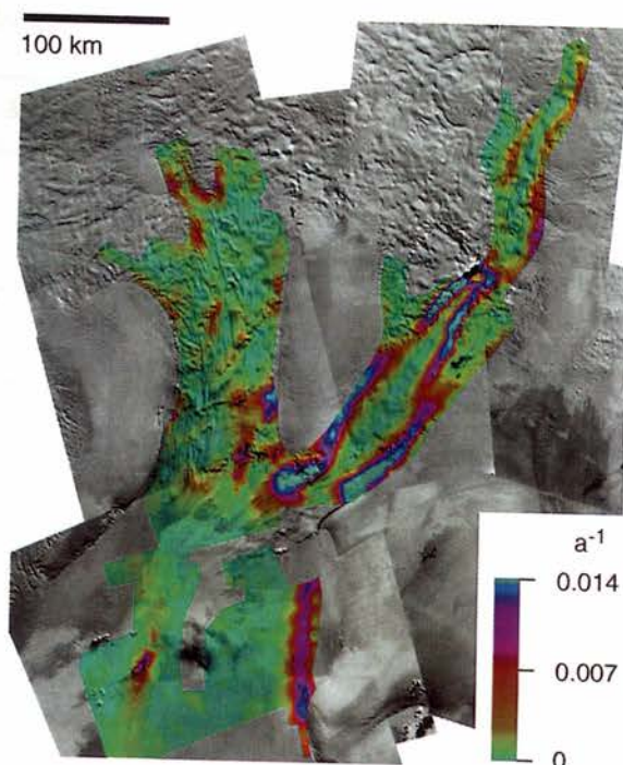
Fig. 7. Shear strain-rate magnitude (color) calculated from velocity data as described in text. Spatial distribution of errors is very similar to that shown in Figure 8.
