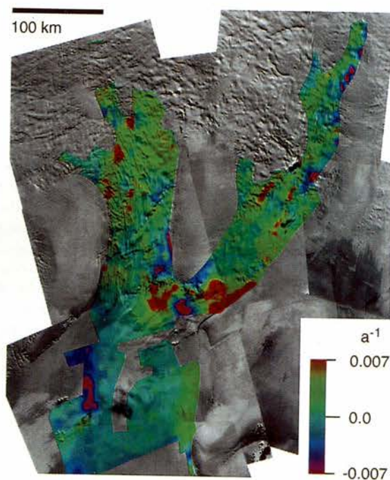
Fig. 5. Longitudinal strain rate (color) calculated from velocity data as described in text. Spatial distribution of errors is shown in Figure 8.
