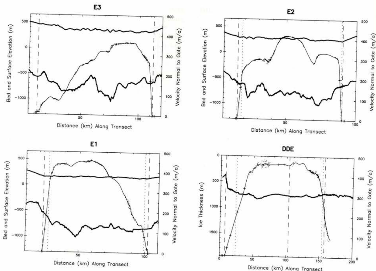
Fig. 10b. Four transects of surface and bed elevations (from airborne radar; heavy lines) and surface velocity (from satellite imagery). See Fig. 10a for description.
