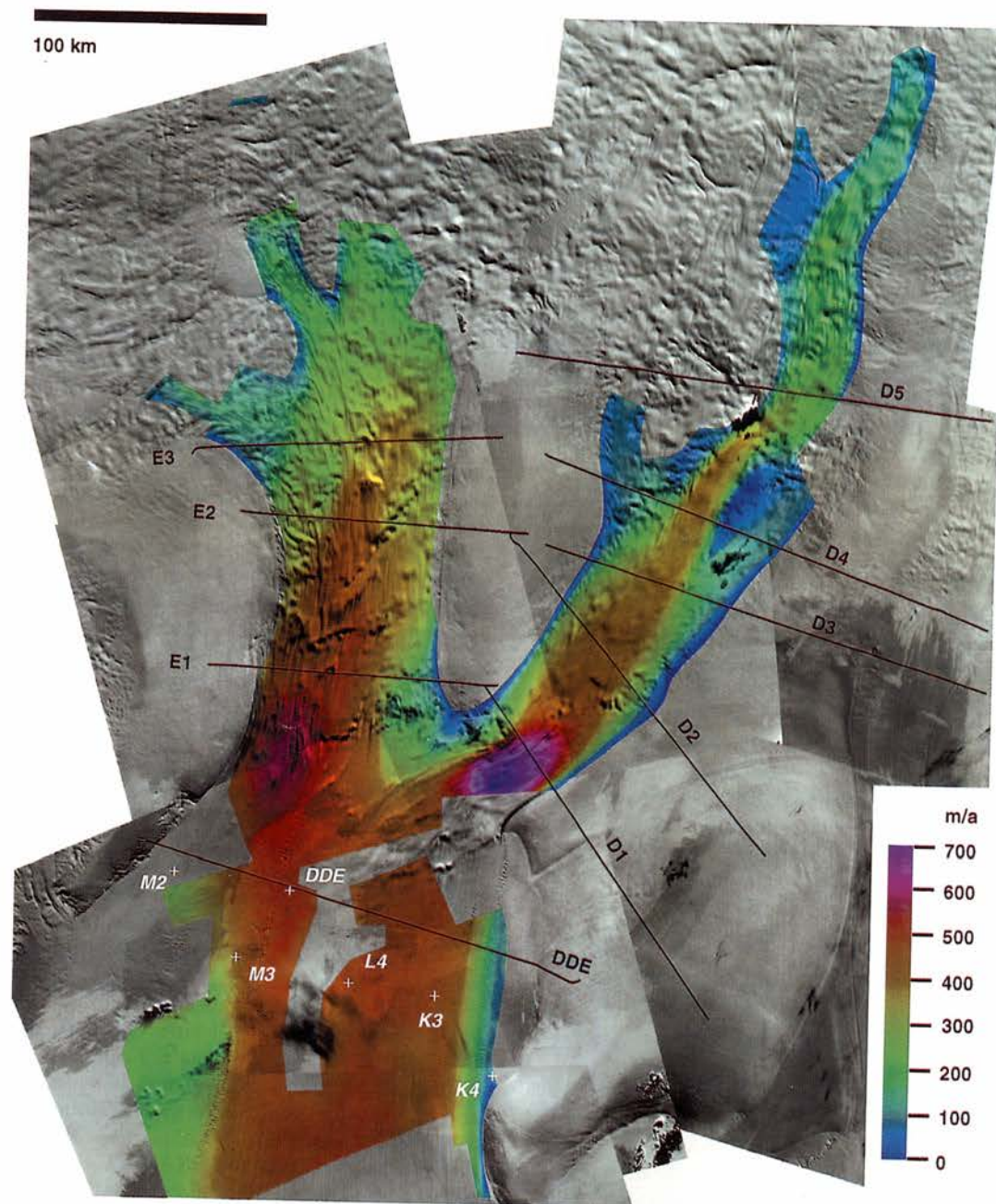
Fig. 4. Color-coded velocity magnitude (speed) superimposed on image mosaic. Transects are shown in black. White crosses show positions of stations discussed in text.
