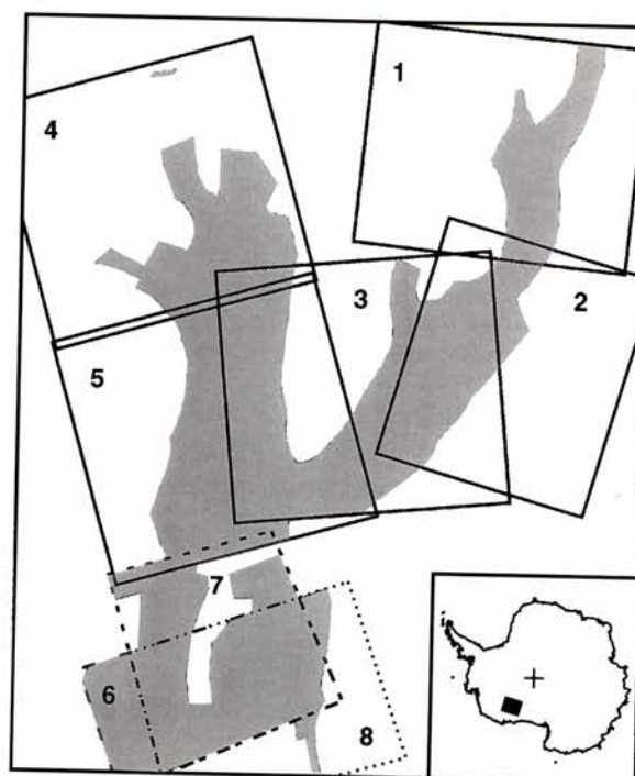
Fig. 2. Location of TM image pairs used in velocity determination. Image ID numbers, acquisition dates and time interval between each image pair are listed in Table 1.
