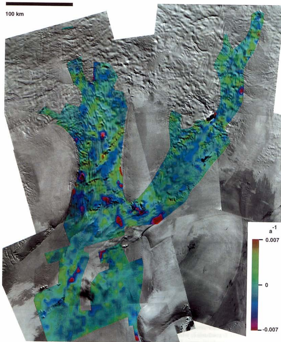
Fig. 9. Color-coded vertical strain rate superimposed on image mosaic. Spatial distribution of errors is very similar to that shown in Figure 8.
