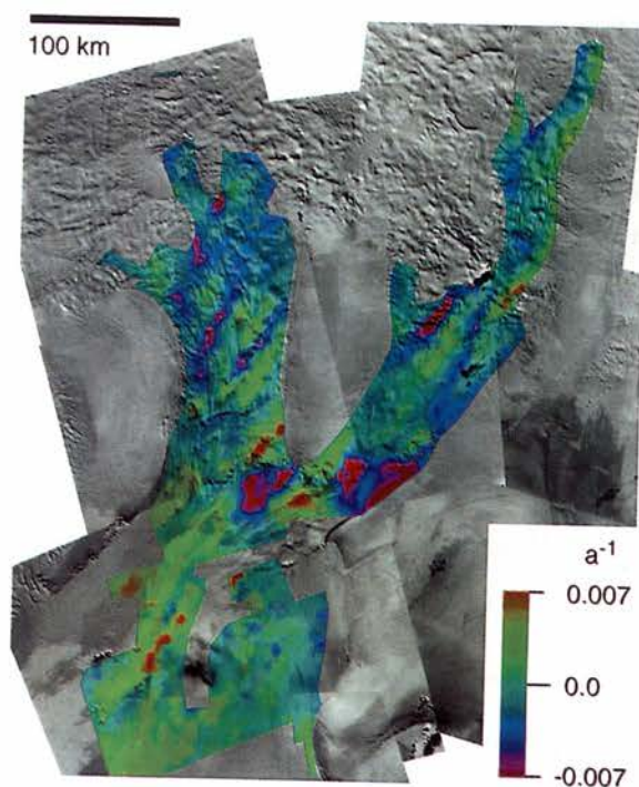
Fig. 6. Transverse strain rate (color) calculated from velocity data as described in text. Spatial distribution of errors is very similar to that shown in Figure 8.
