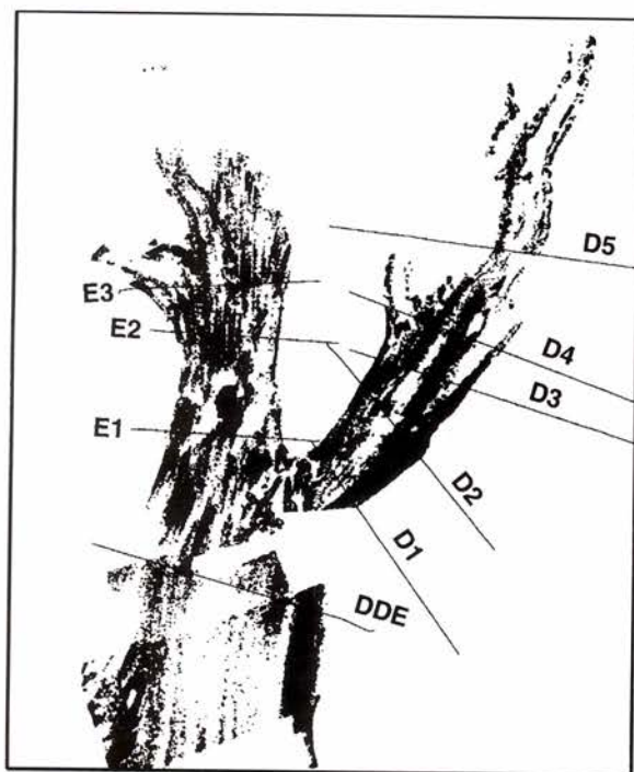
Fig. 3. Positions of 75 382 velocity data points determined by cross-correlation technique and positions and names of airborne transects.
