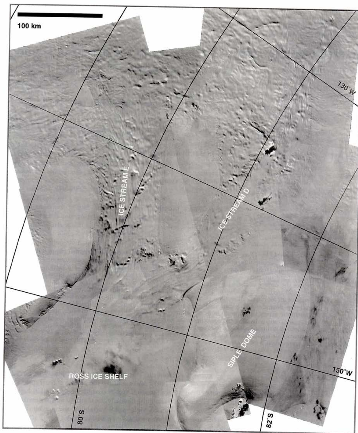
Fig. 1. Image mosaic of Ice Streams D and E using ten Landsat TM scenes. See Figure 2 for location of this region.
