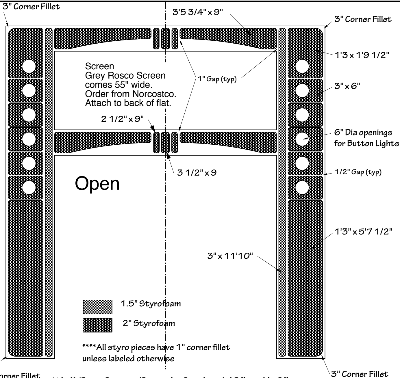
Wall Box Styro Detail Scale: 1/2" = 1'-0"
