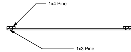
Top View Detail Unit T - Typical for Units A through U and Backup Singer Platforms Scale: 1/2" = 1'-0"
