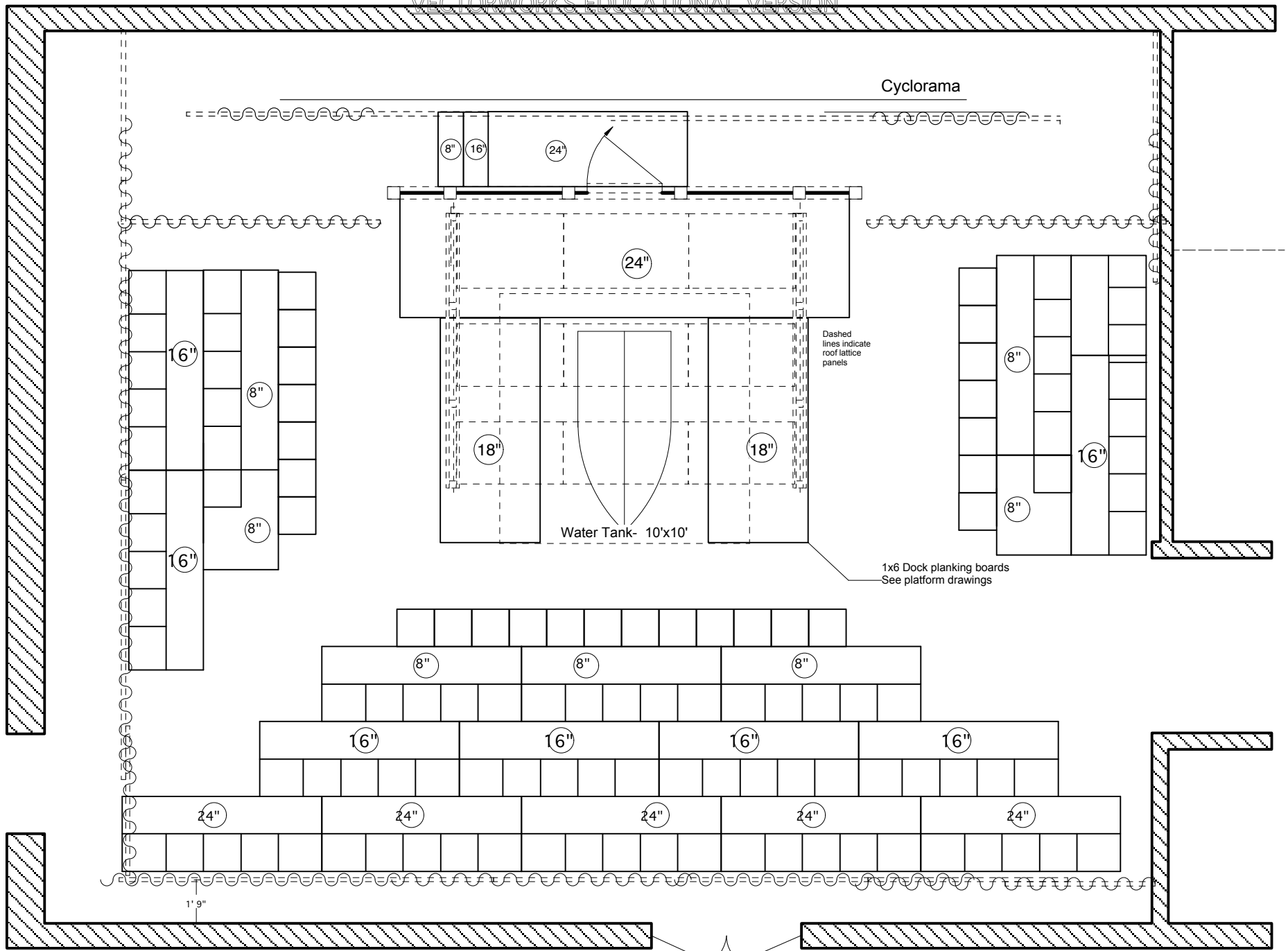
Talley's Folly Floorplan Scale: 3/16"=1'-0" 7/30/15 B. Bjorklund
