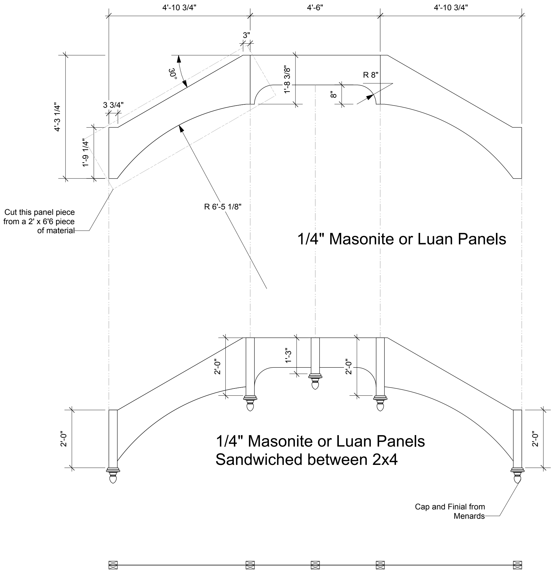
Top View
