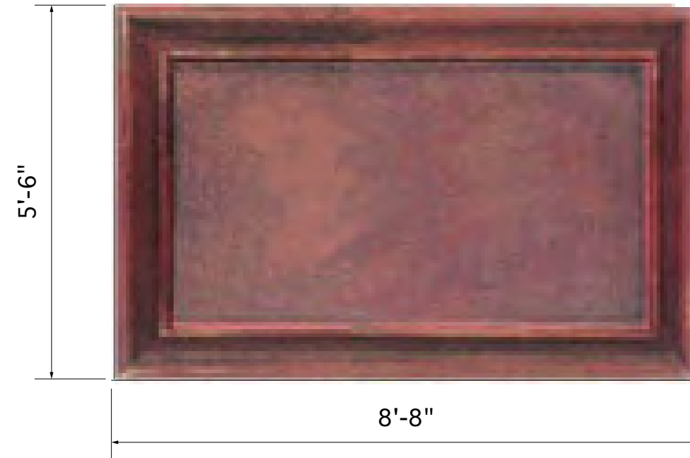
Projection Panels- Make 2 Mount on Proscenium Wall L&R. See Scenic Model
