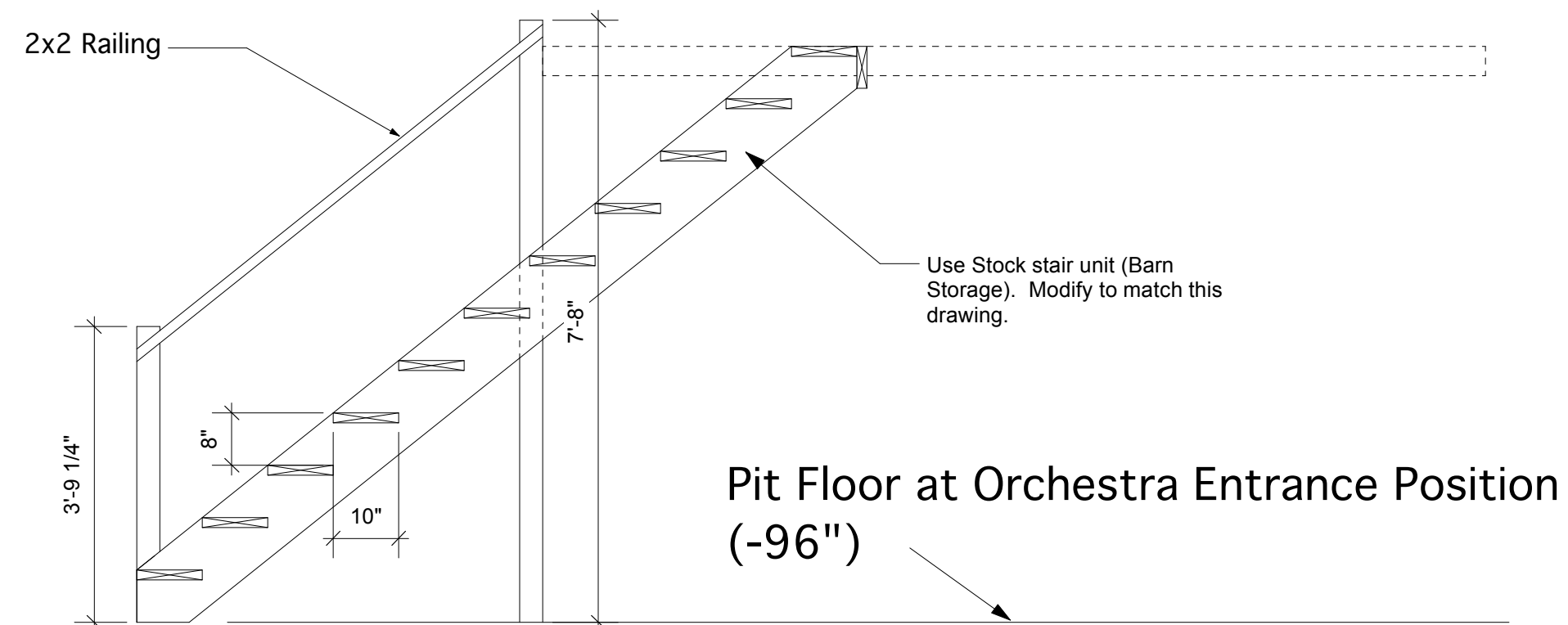
Section View: B-B'
