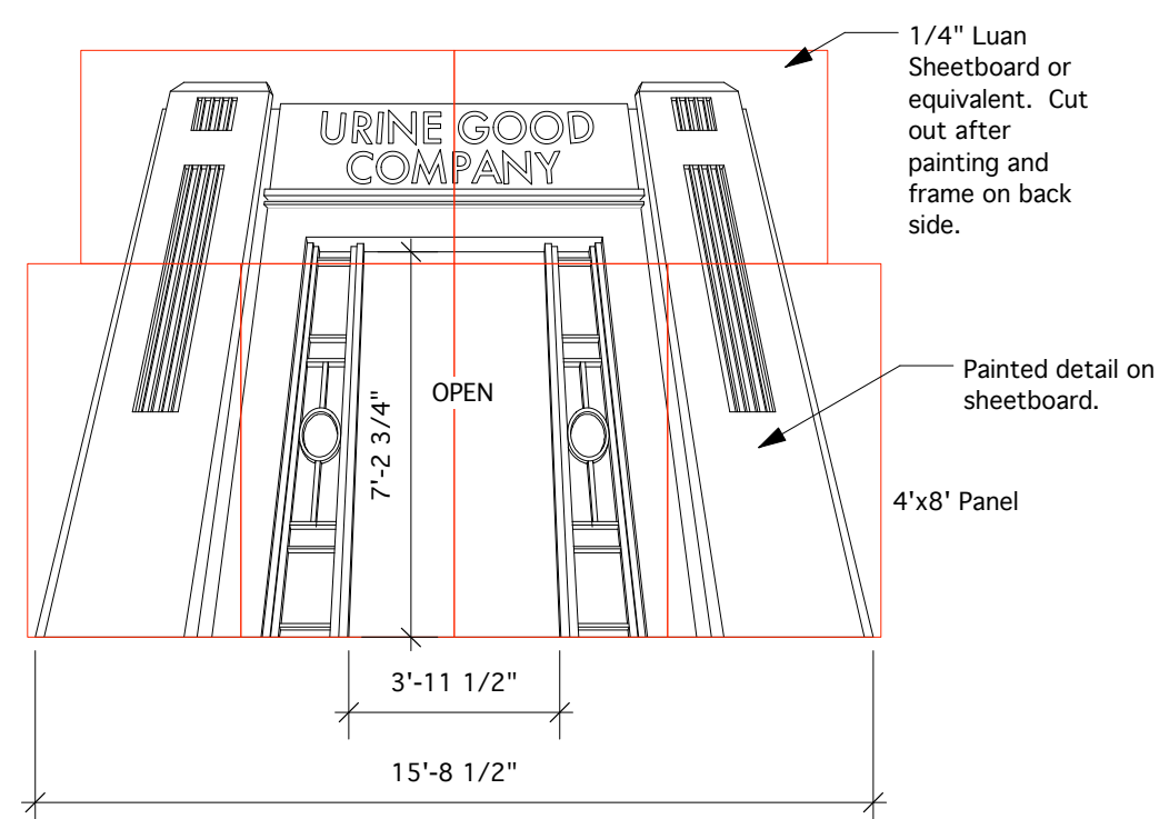
Lower UGC Building Panel Line 10
