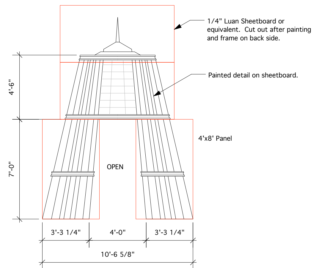
Upper UGC Building Panel Line 16
